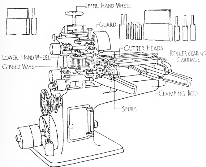
FIG. 196. TENONING MACHINE.
